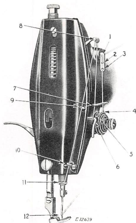
Fig.15. Upper Threading
