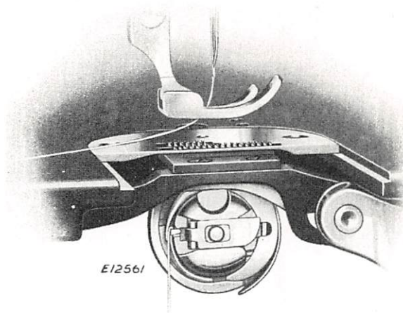
Fig. 14. Bobbin Case Threaded and Replaced
