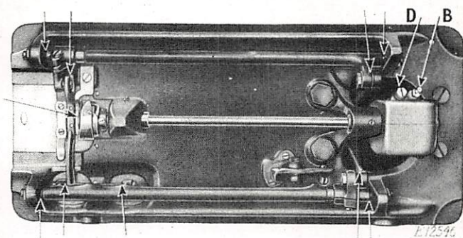
Fig. 6. Oiling Points in Base of Machine
