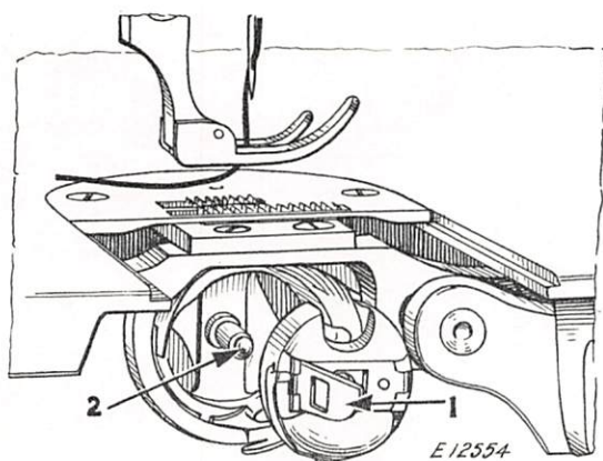
Fig.9. Removing the Bobbin
