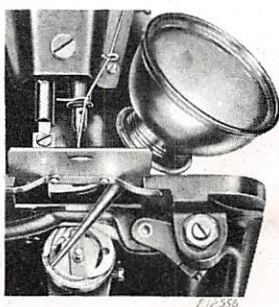
Fig. 7. Oiling Point in Hook Race
